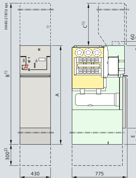
Bus sectionalizer panel type H with switch-disconnector/fuse combination
