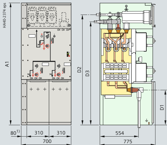
Panel block RRT compact
