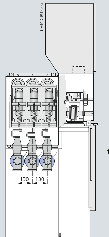
1 Bus / cable-type current transformer 4MC70 32
