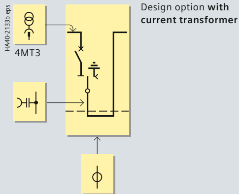
Type V (with circuit- breaker 1.1 or 2) 500 mm wide
