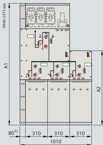
Panel block RRT-R Compact
