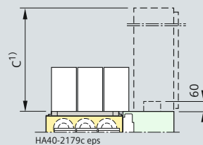
Design option with busbar voltage transformer for all circuit-breaker types
