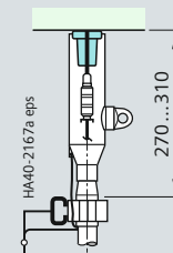
Cable routing downwards with straight plug
