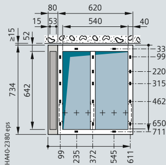
Panel block RRT Compact
