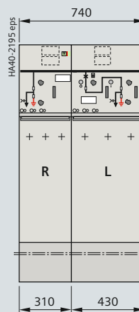
Panel block RL
