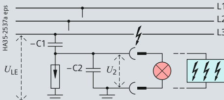
LRM system CAPDIS/VOIS plugged in installed
