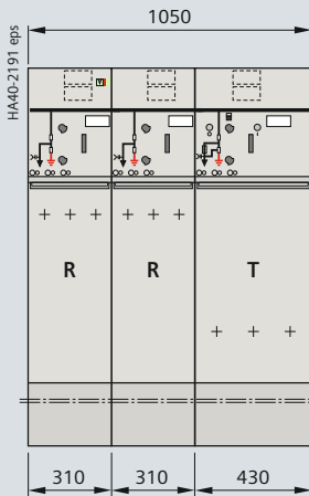
Panel block RRT
